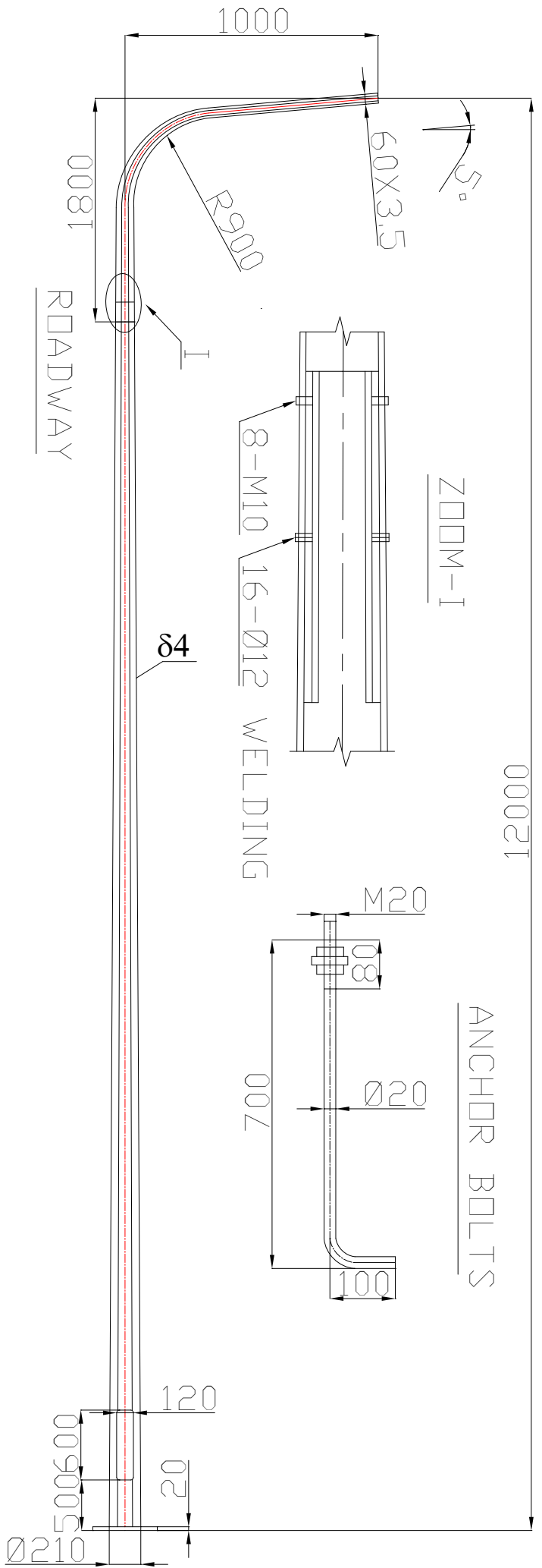
OCTAGONAL SINGLE ARM POLE
